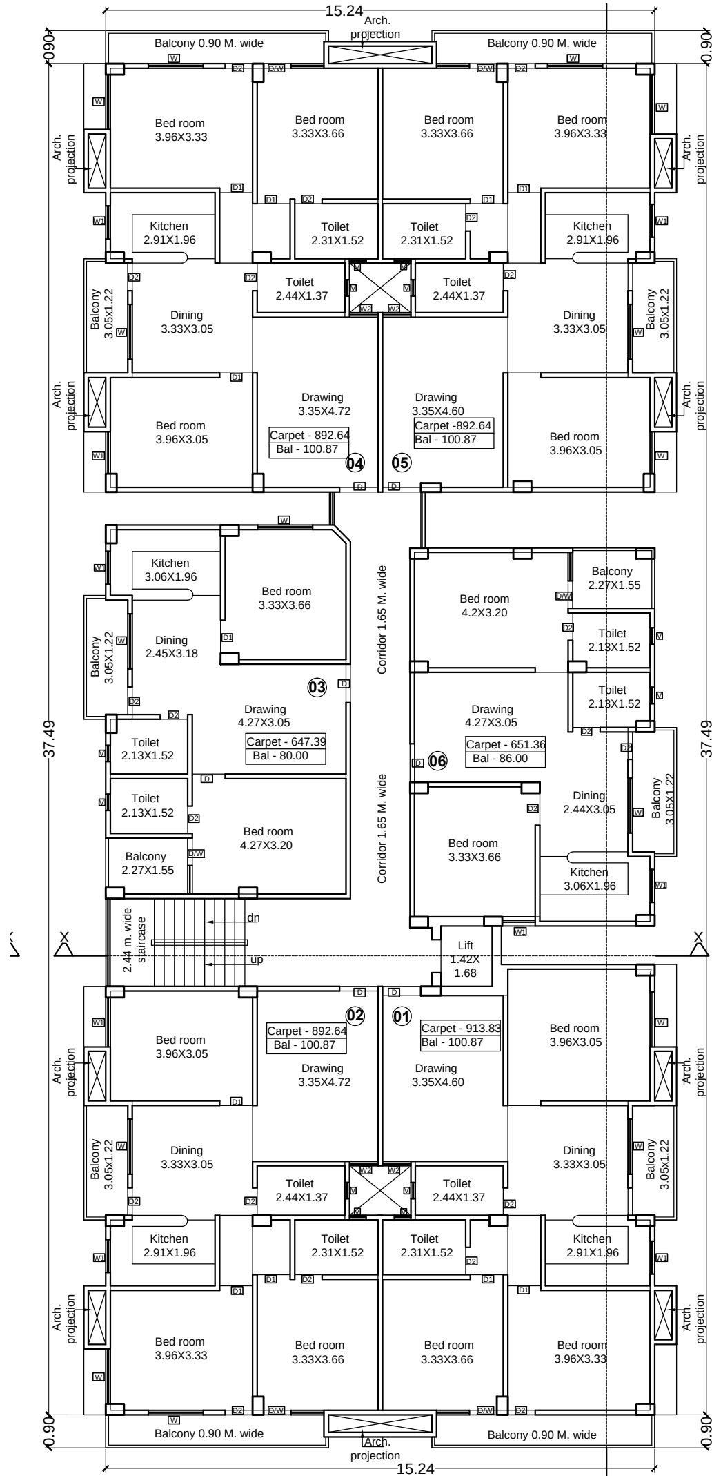
TYPICAL(1st to 4th.) FLOOR PLAN SCALE:1=100
