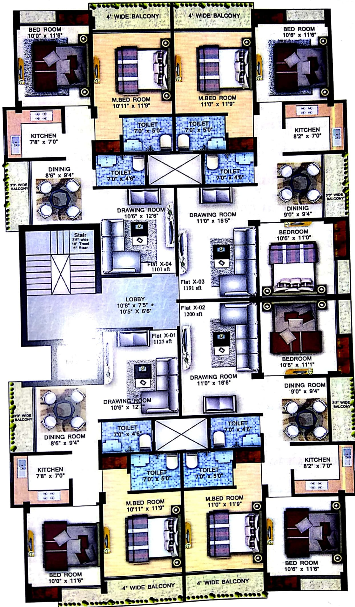
TYPICAL FLOOR PLAN BLOCK 11
