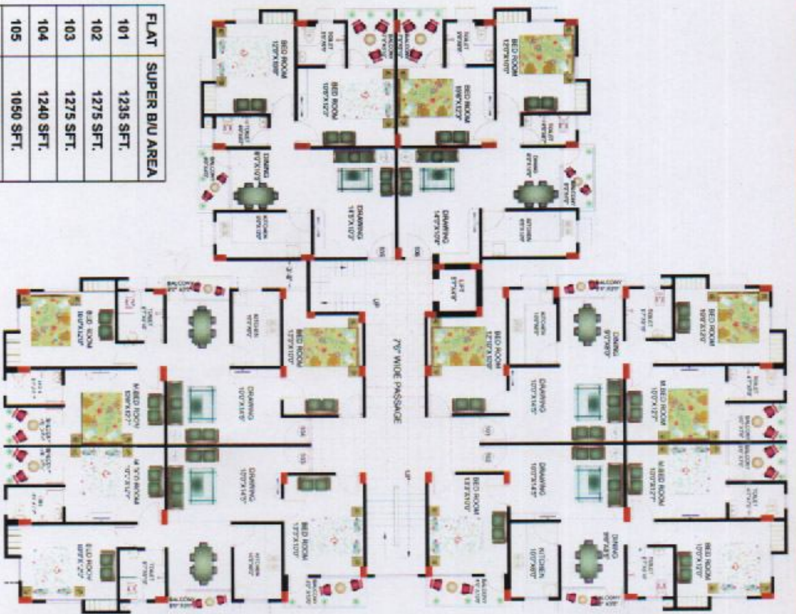
TYP.1ST.TO 4TH. FLOOR PLAN
