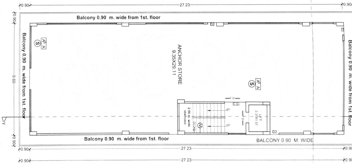
TYPICAL (1ST. TO 4TH.) FLOOR PLAN SCALE :- 1 = 100
