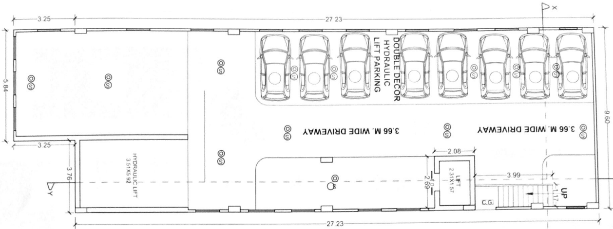
BASEMENT FLOOR PLAN SCALE :- 1 = 100
