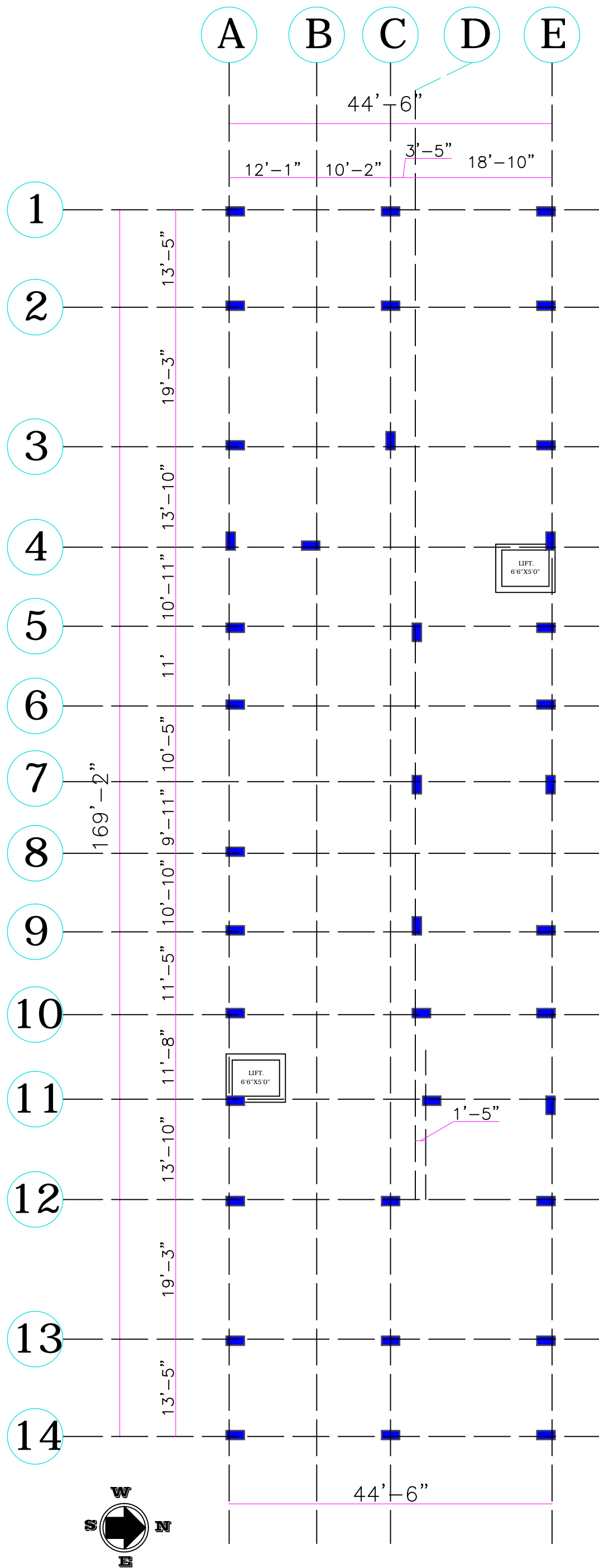
COLUMN LAY-OUT PLAN
