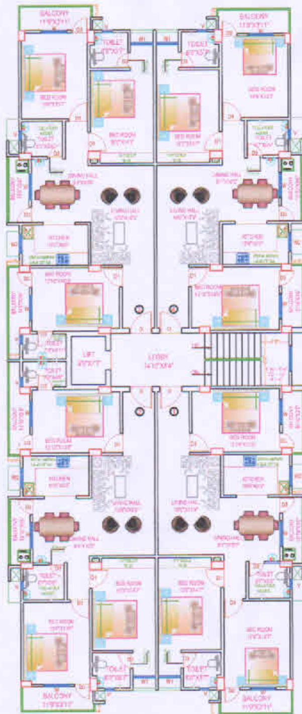
TYPICAL 1ST TO 4TH FLOOR PLAN.
