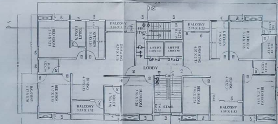
4TH & 5TH FLOOR PLAN
