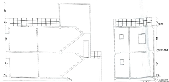
SECTION: X-X (SCALE: 1:100)
