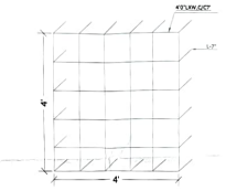
DETAILS OF CAP NET IN FOUNDATION
