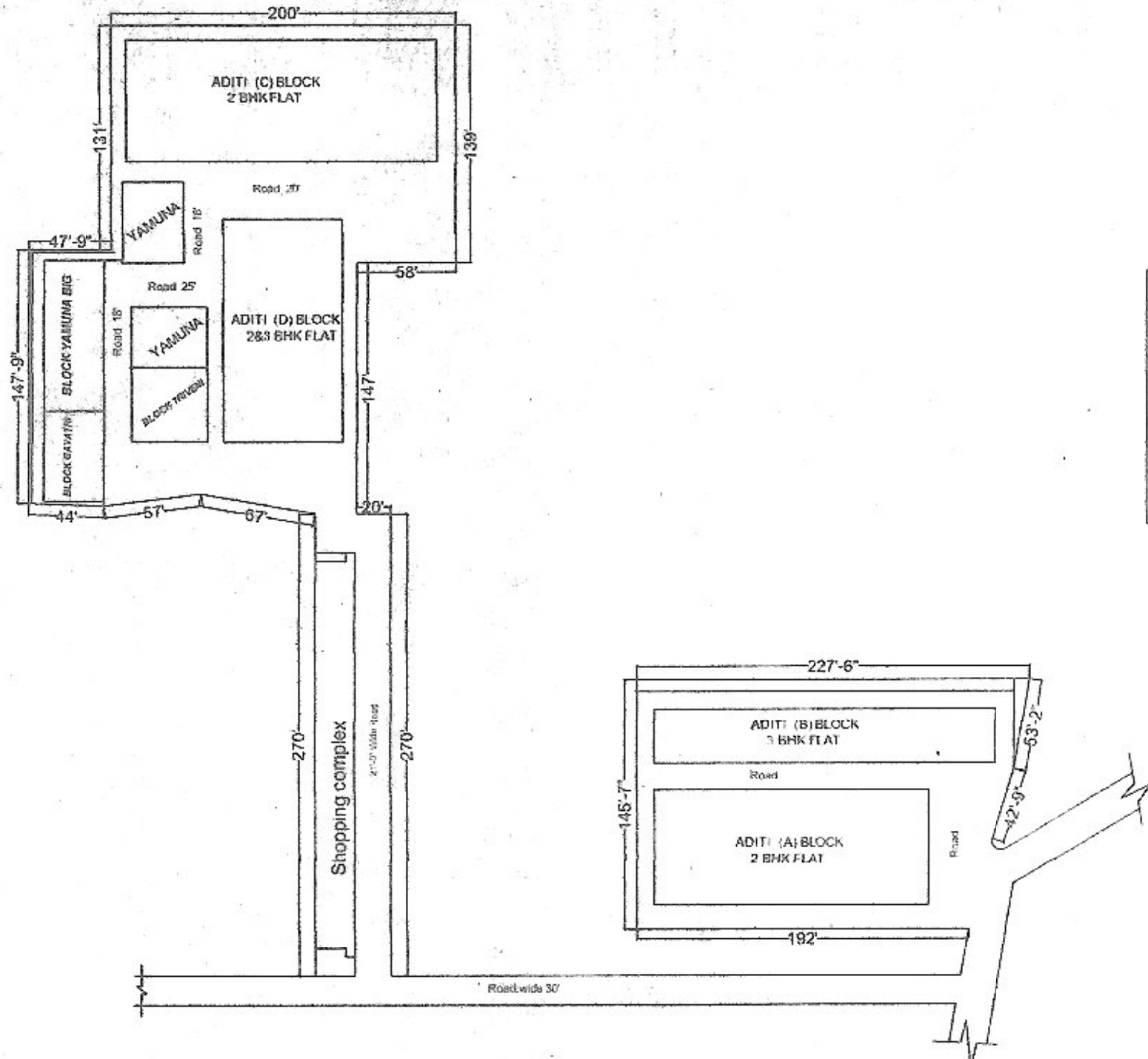
BLOCK PLAN
