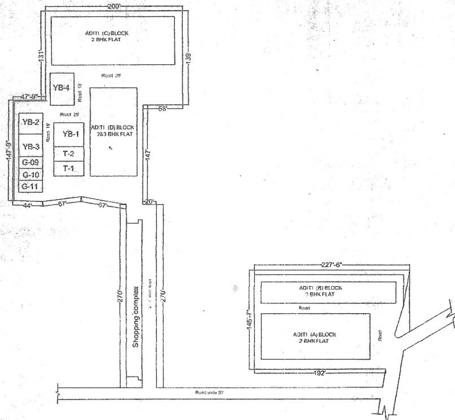
UNITS PLAN
