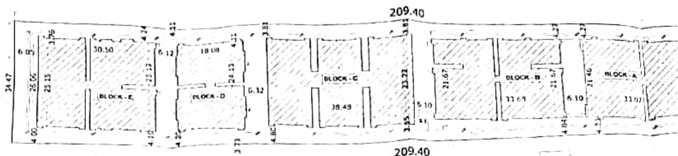
SITE PLAN
