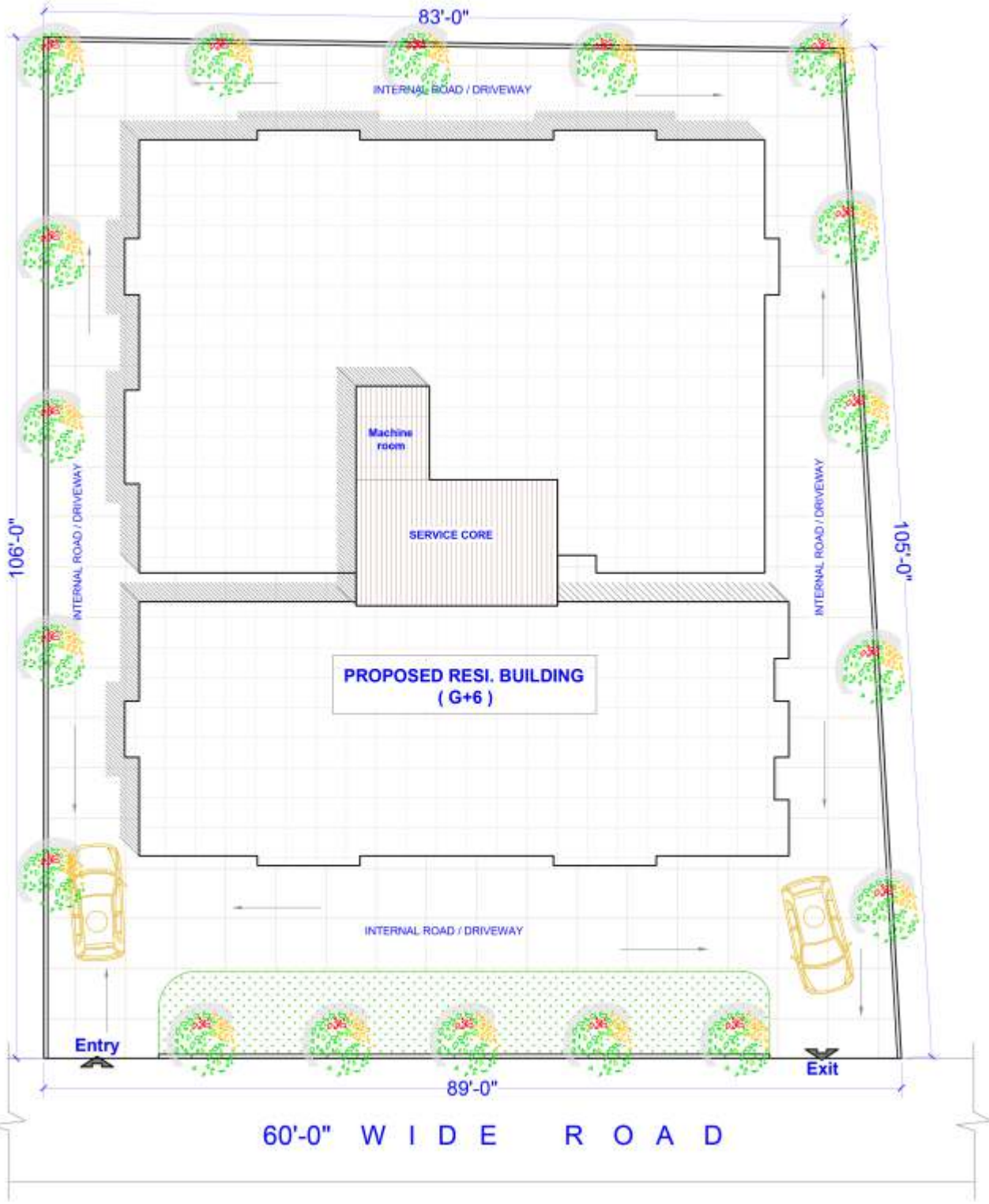
SITE PLAN
