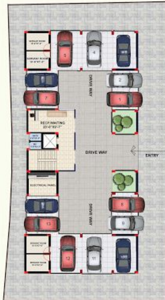
GROUND FL. PLAN
