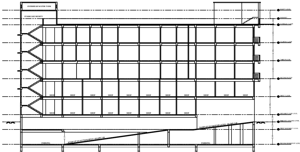
SECTION - YY'
