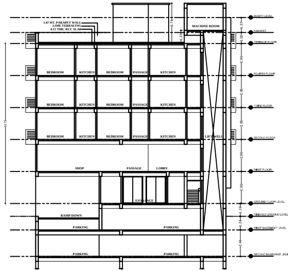
SECTION - XX'
