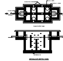
DETAILS OF SEPTIC TANK
