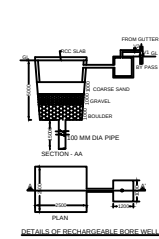
DETAILS OF RECHARGEABLE BORE WELL
