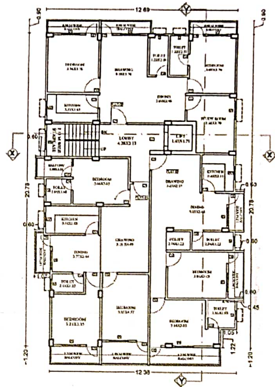
2ND TO 4TH FLOOR PLAN
