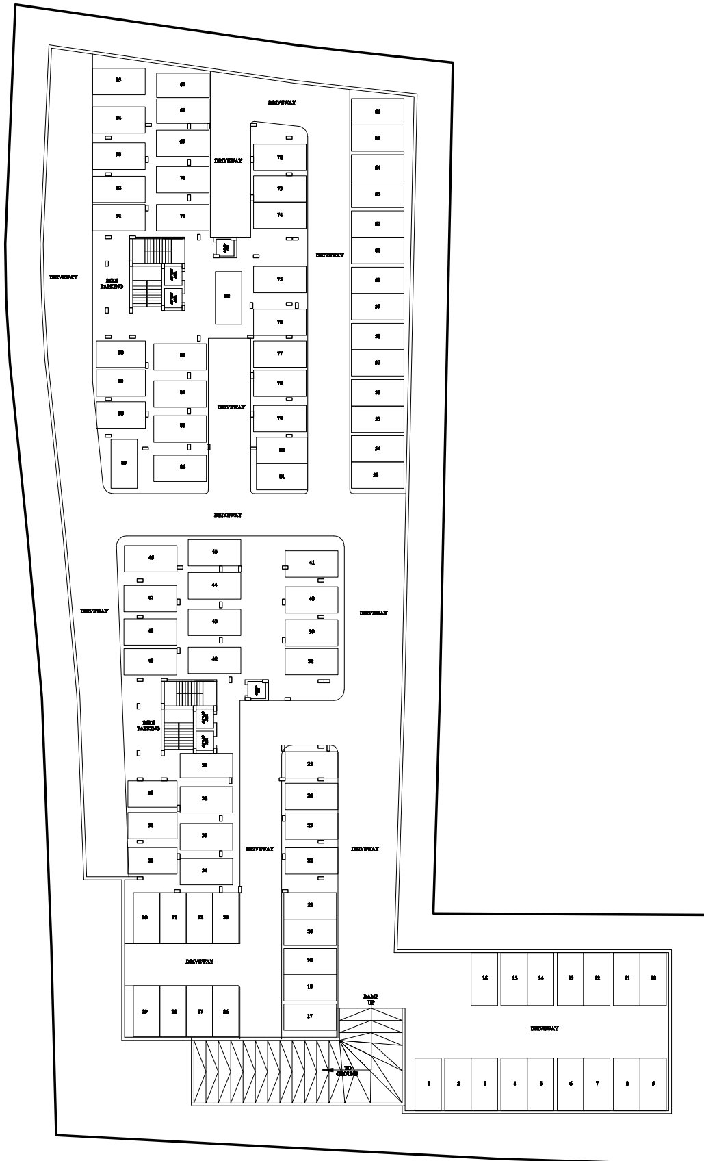
BASEMENT PARKING PLAN
